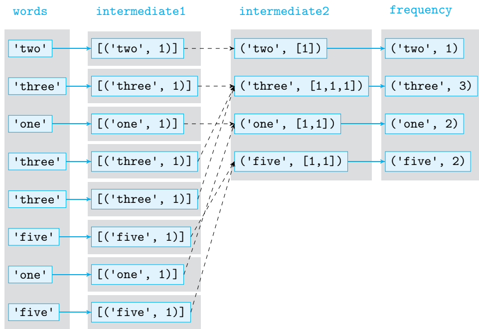
Figure 12.13 MapReduce for word frequency. List comprehension is used to map each word in list words to a list [(word,1)]. Those new lists are stored in list intermediate1. Then all [(word,1)] lists of intermediate1 containing the same word are pulled together to create tuple (word, [1,1,...,1]). In the last step, the 1s in every such tuple are added up into variable count, and tuple (word, count) is added to list frequency.
